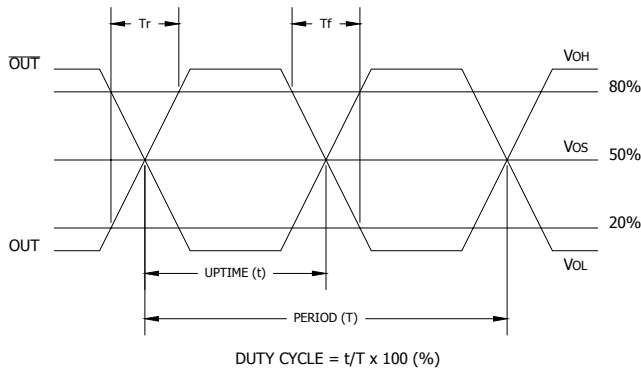
PECL/LVDS OUTPUT WAVEFORM
