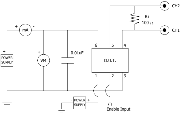
TEST CIRCUIT, LVDS LOAD
